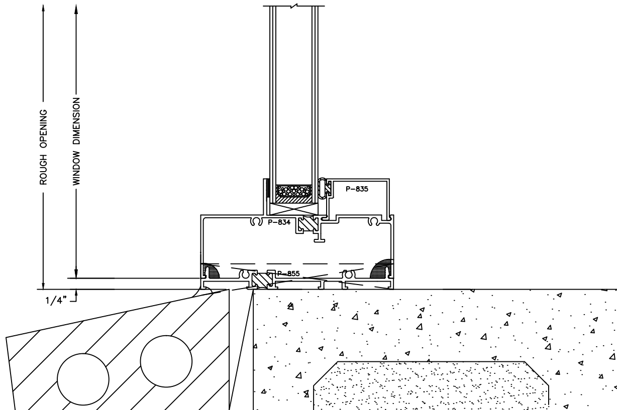
SILL STARTER FOR 4" WINDOW SYSTEMS
