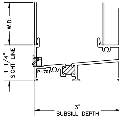
HIGH PERFORMANCE SUBSILL
