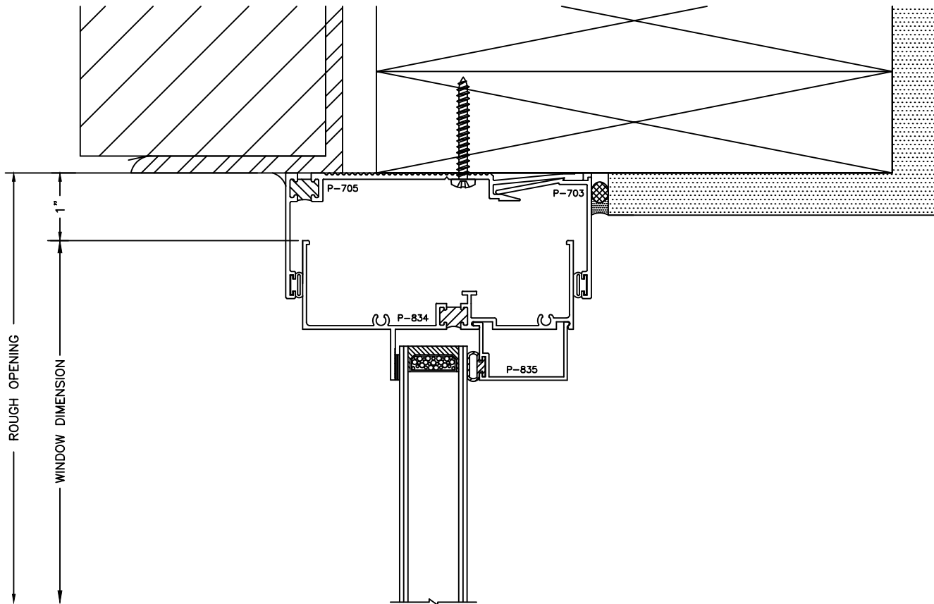
RECEPTOR FOR 4" WINDOW SYSTEM
