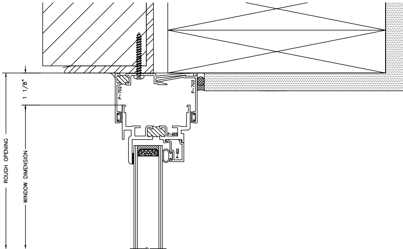
RECEPTOR FOR 2 3/8" WINDOW SYSTEMS
