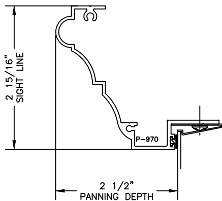
P-970 HISTORICAL PANNING
