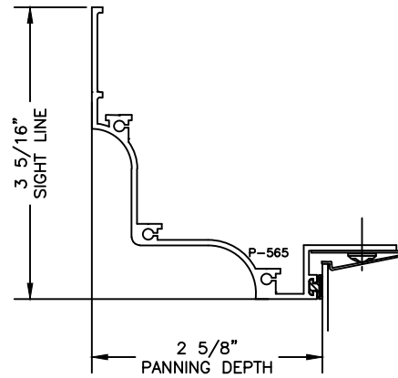
P-565 HISTORICAL PANNING
