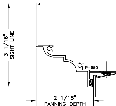
P-950 HISTORICAL PANNING
