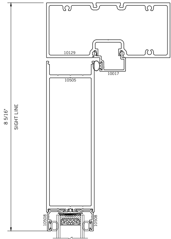
1" INSULATED GLASS
