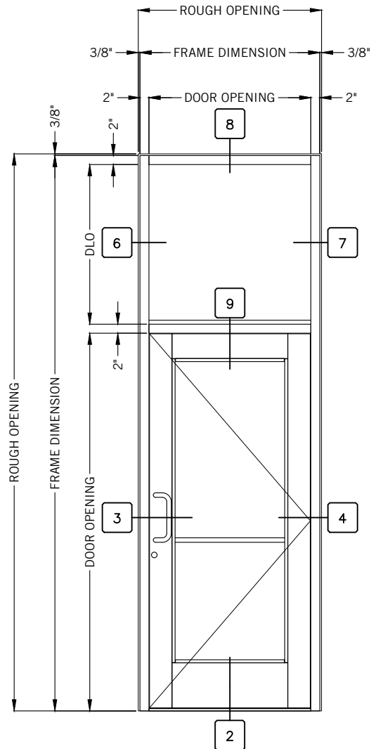
WIDE STILE W/ TRANSOM
