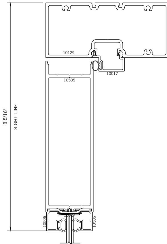
1/4" SINGLE GLAZED
