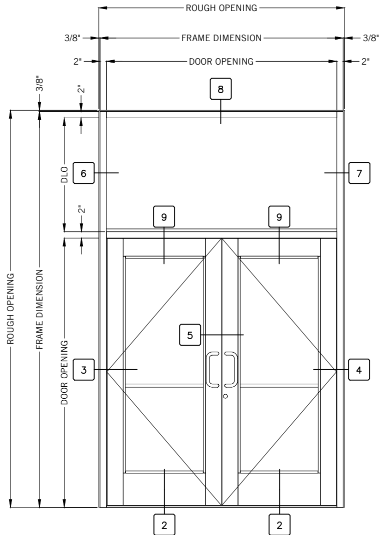
WIDE STILE PAIR W/ TRANSOM
