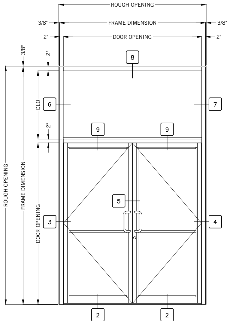
NARROW STILE PAIR W/ TRANSOM
