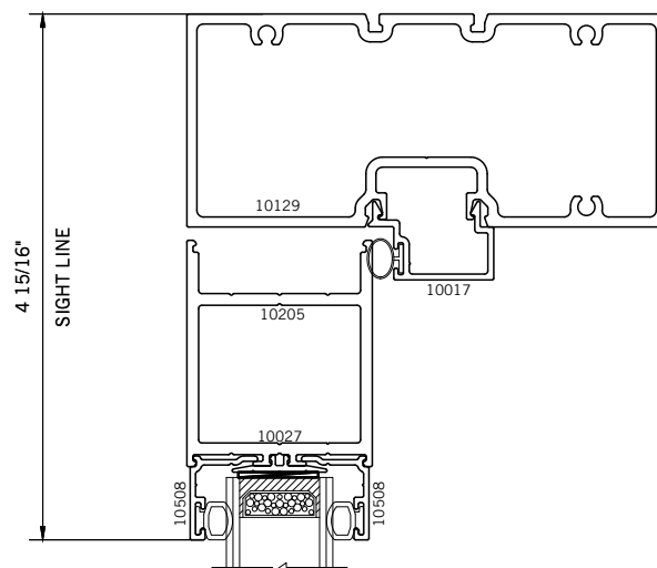
1" INSULATED GLASS
