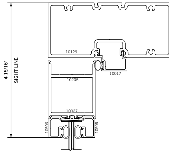
1/4" SINGLE GLAZED
