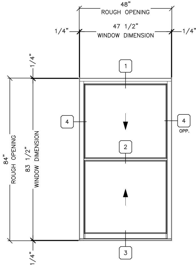
DOUBLE HUNG
