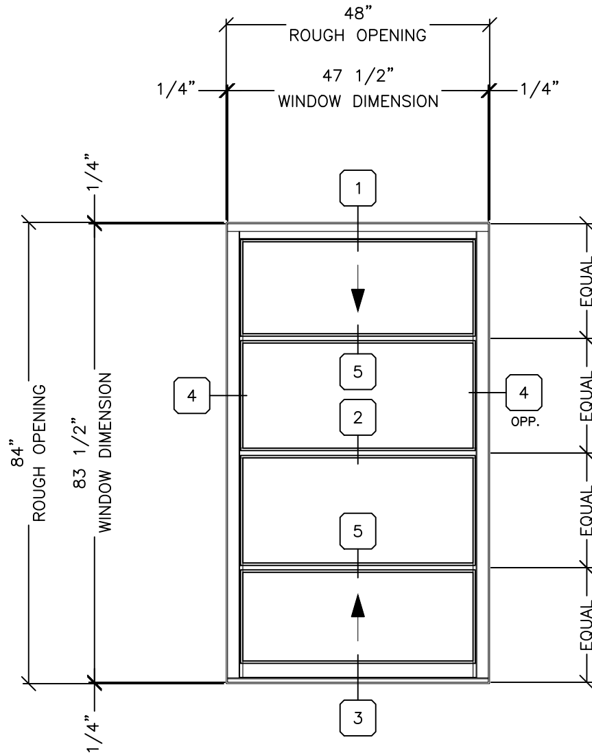
DOUBLE HUNG WITH TRUE MUNTIN
