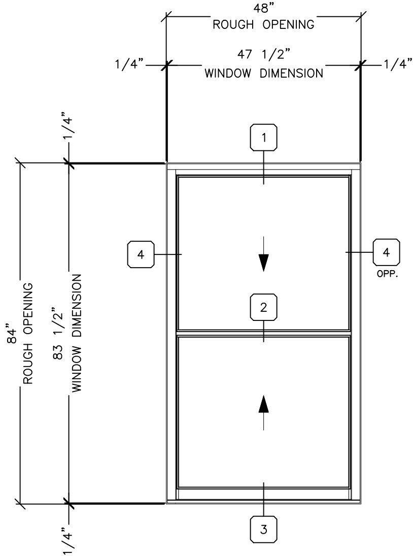
DOUBLE HUNG
