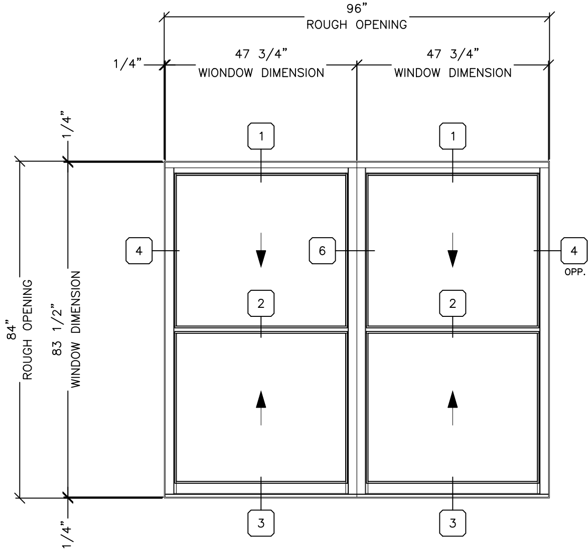
DOUBLE HUNG / DOUBLE HUNG
