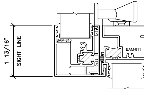
SWEEP LOCK
