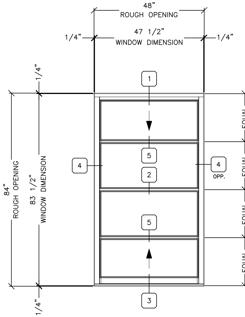
DOUBLE HUNG WITH TRUE MUNTIN
