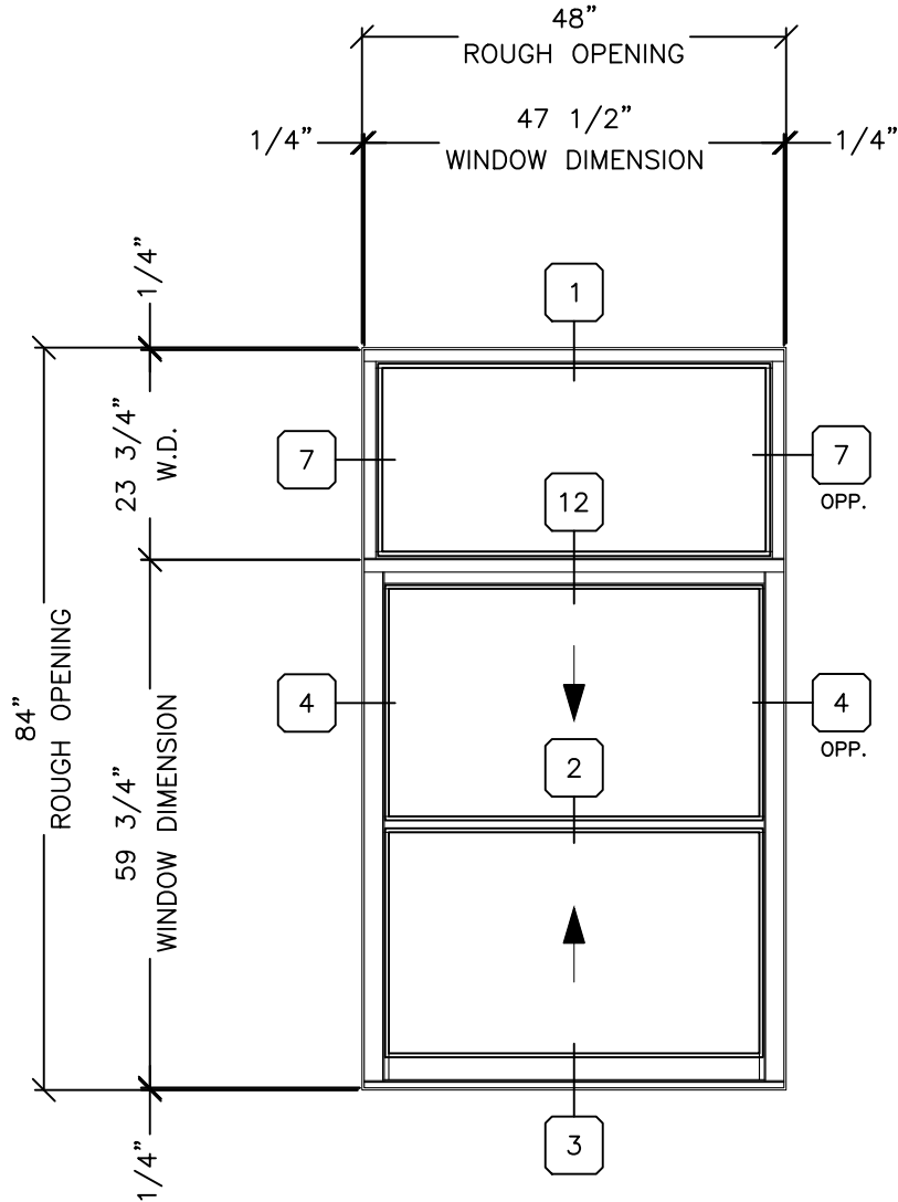
FIXED / DOUBLE HUNG TWO PIECE STACK
