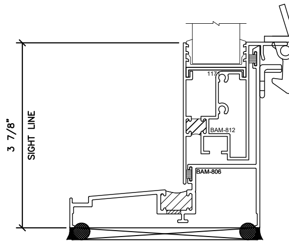
AUTO SILL LOCK
