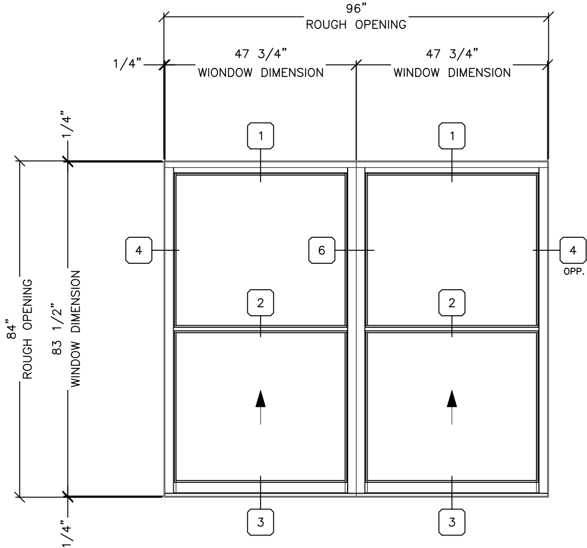
SINGLE HUNG / SINGLE HUNG
