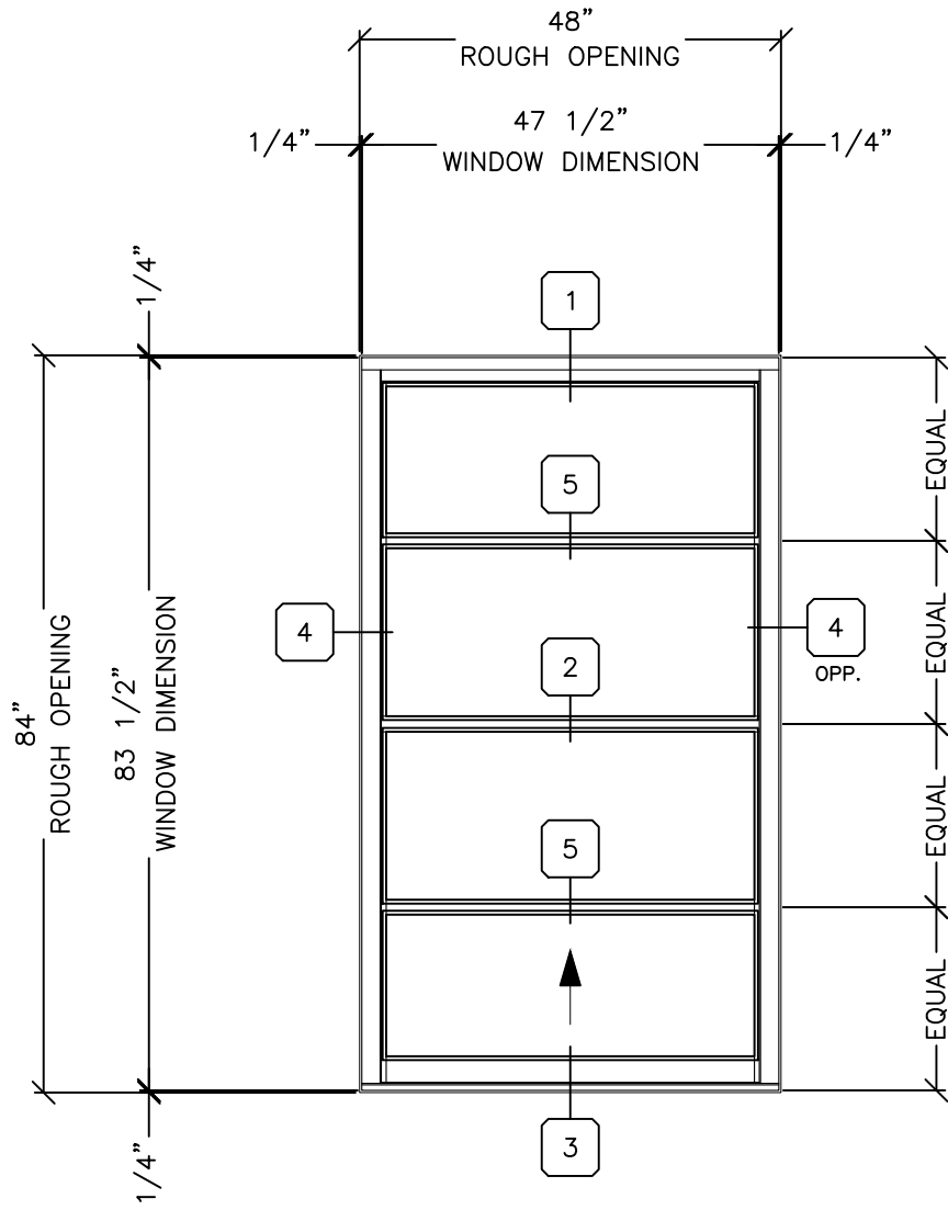
SINGLE HUNG WITH TRUE MUNTIN
