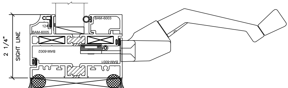
ROTO-OPERATOR
