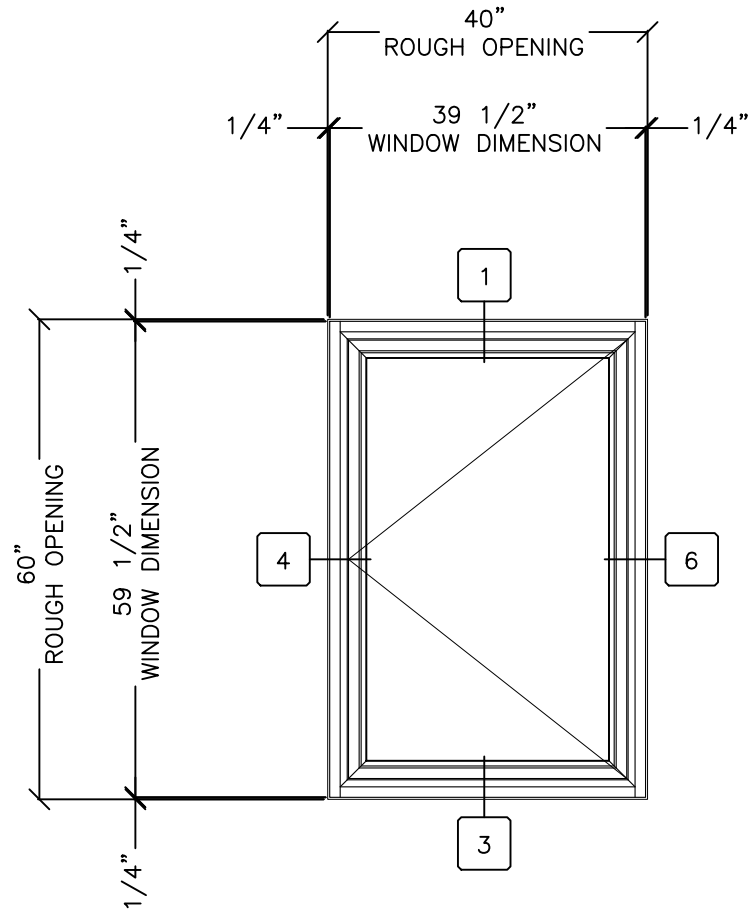
CASEMENT
