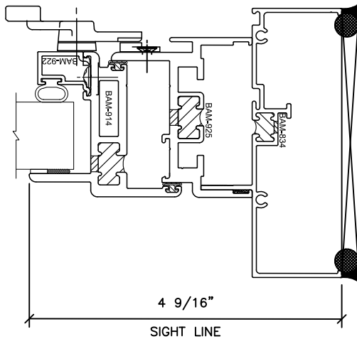
CAM LATCH
