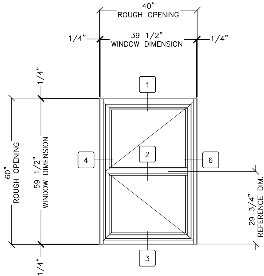
CASEMENT WITH TRUE MUNTIN
