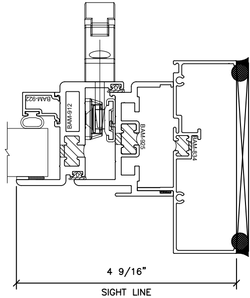
MULTI POINT LATCH
