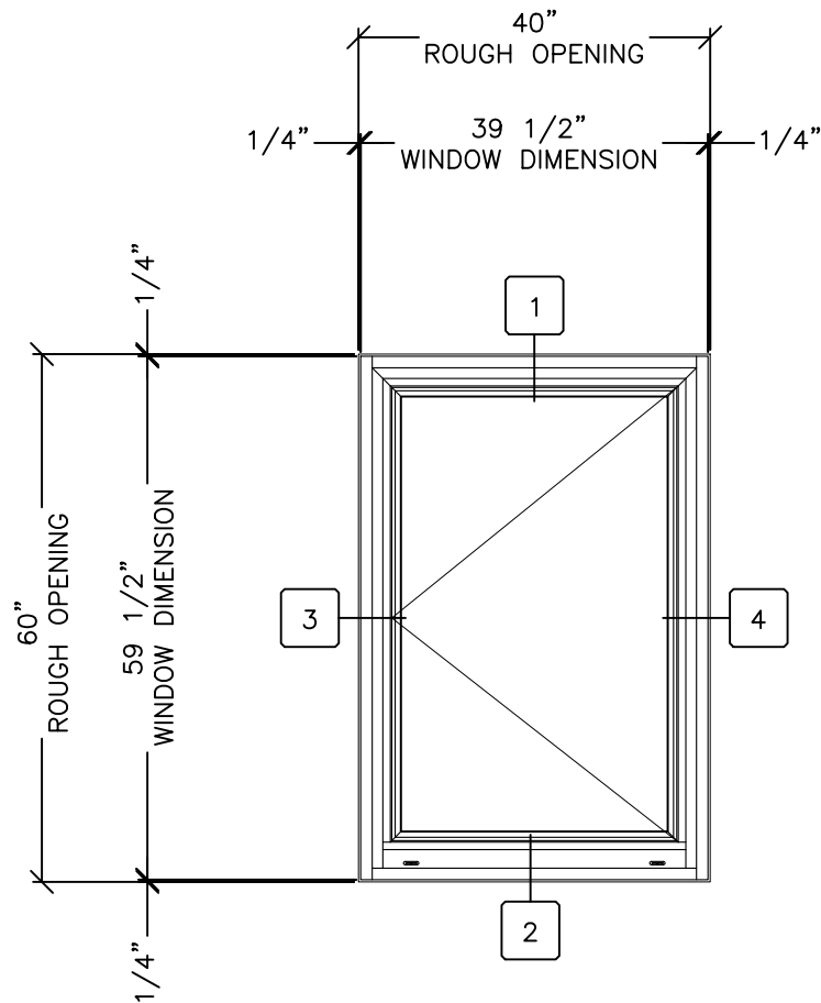
INSWING CASEMENT
