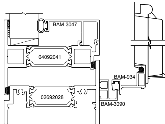
SILL
