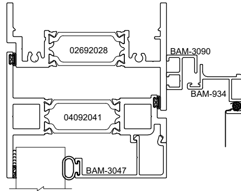
HEAD
