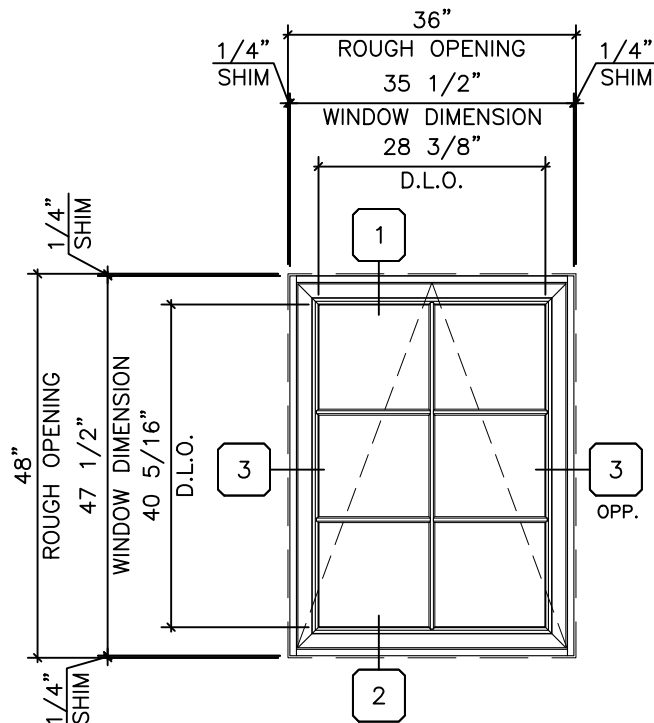
PROJECT OUT W/ GRID
