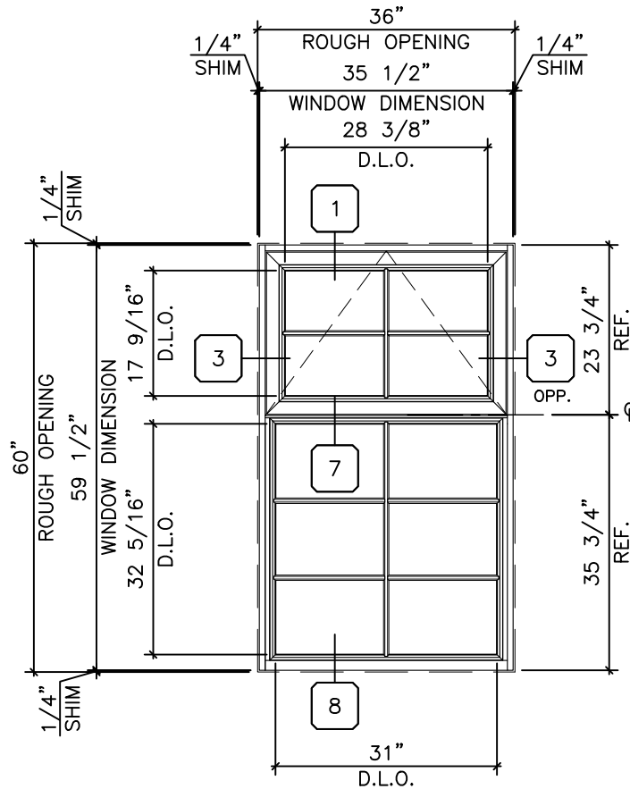
PROJECT OUT / FIXED W/ GRID
