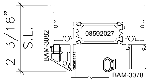
1" UNIT
