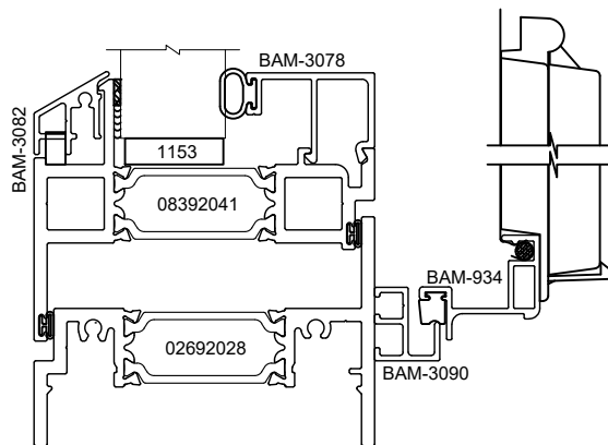
SILL
