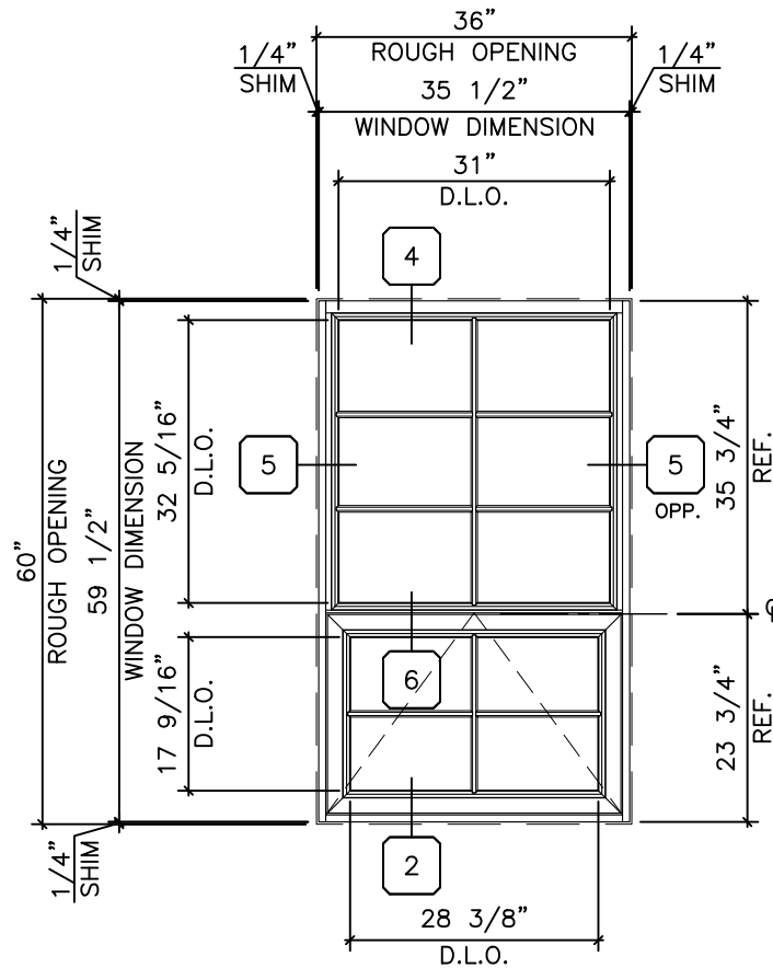
FIXED / PROJECT OUT W/ GRID
