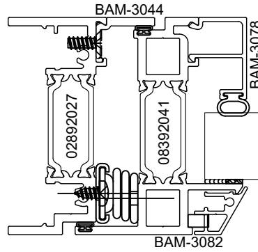
4-BAR ARM
