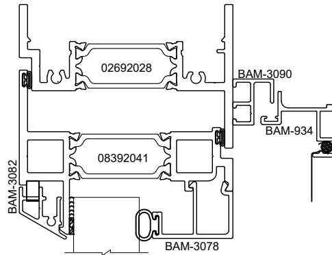
HEAD
