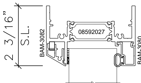
1 3/4" UNIT
