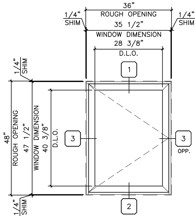
CASEMENT
