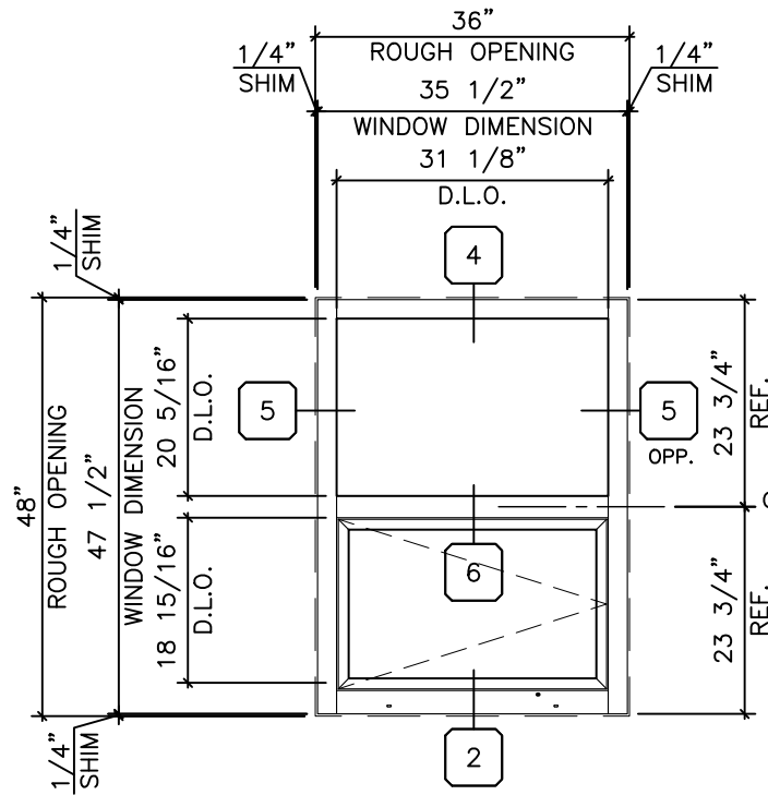
FIXED / CASEMENT
