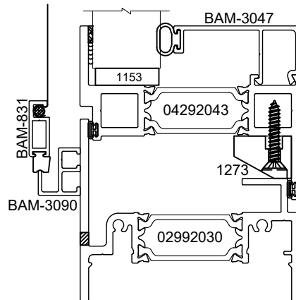
SILL
