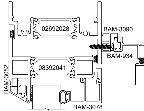
HEAD
