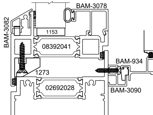
SILL
