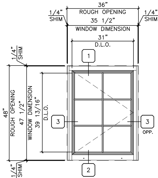
CASEMENT W/ GRID
