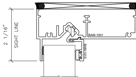
1 1/4" INSULATED GLASS
