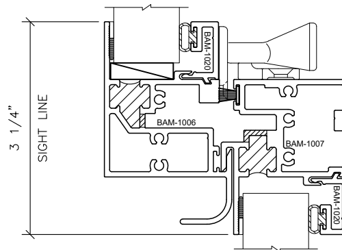
SWEEP LOCK
