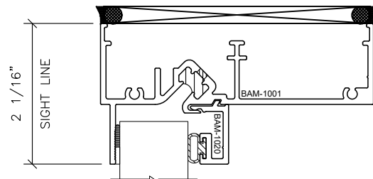
1" INSULATED GLASS
