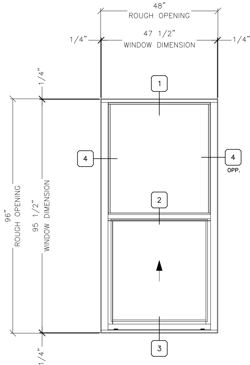
SINGLE HUNG
