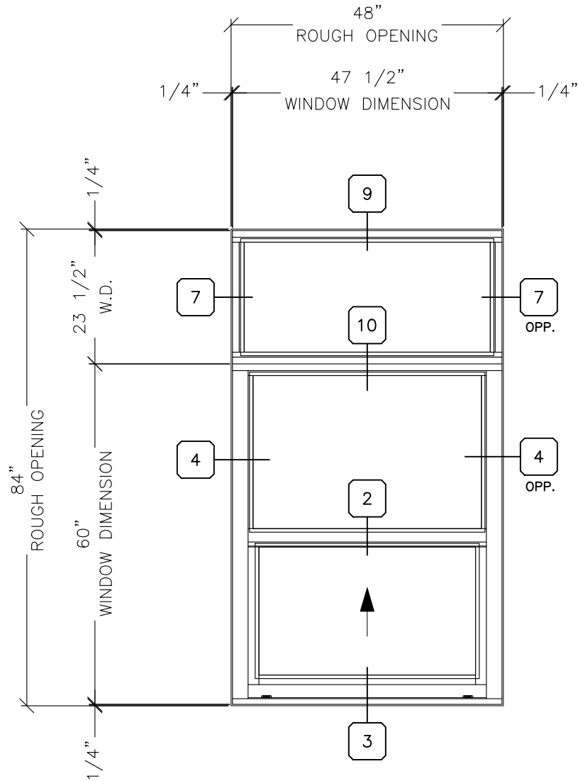
FIXED / SINGLE HUNG TWO PIECE STACK
