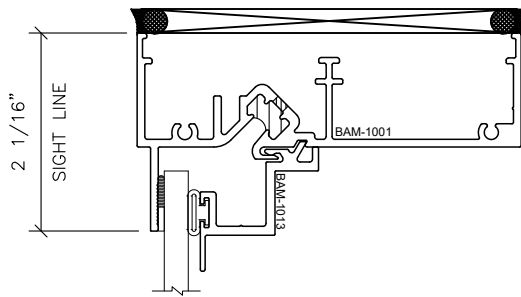
1/4" SINGLE GLAZED
