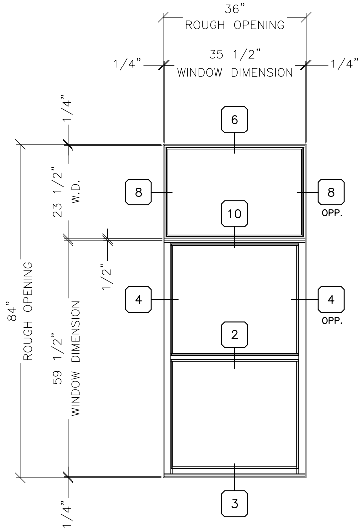
FIXED / SINGLE HUNG TWO PIECE STACK
