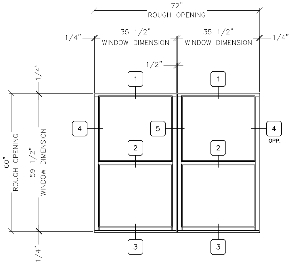
SINGLE HUNG / SINGLE HUNG
