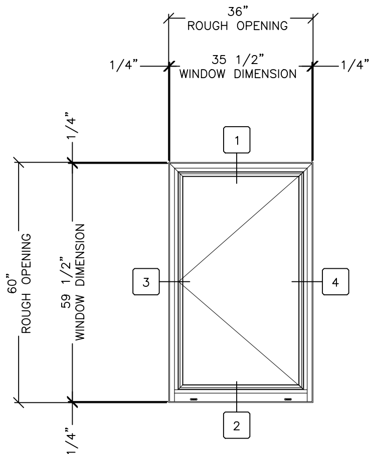
CASEMENT INSWING
