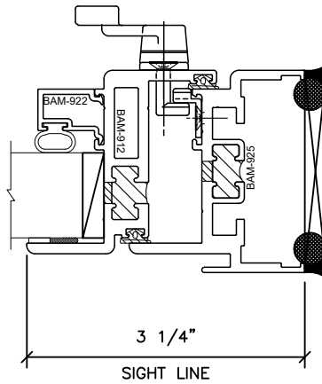
CAM LATCH
