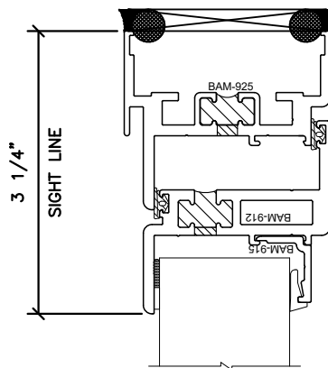
1 1/2" UNIT
