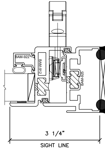
MULTI POINT LATCH
