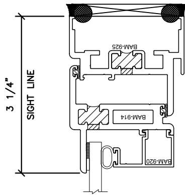
1/4" UNIT
