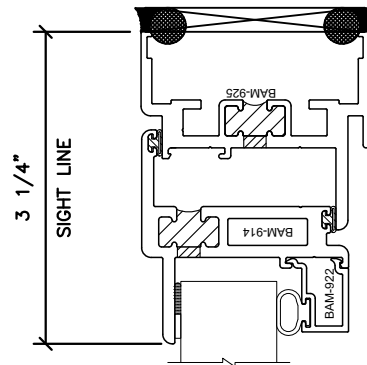
1" UNIT
