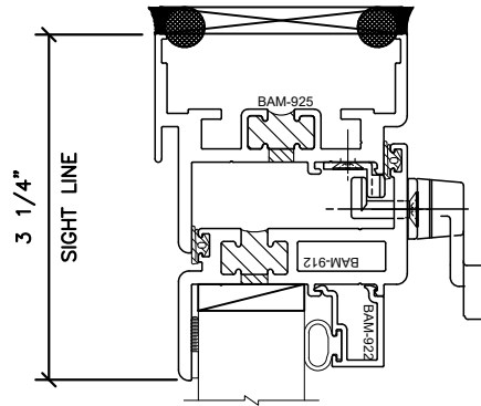
CAM LATCH
