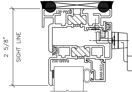
CAM LATCH
