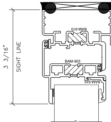
1 1/2" UNIT
