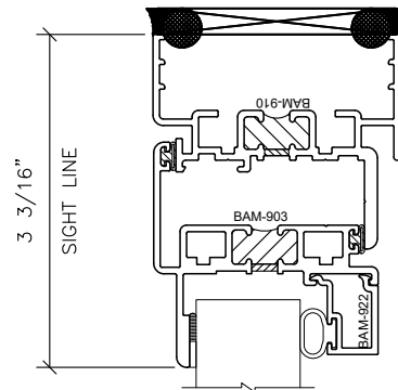
1" UNIT
