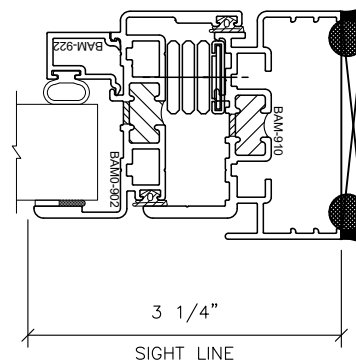
4-BAR ARM
