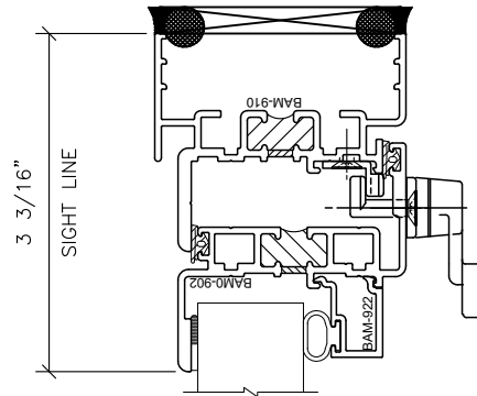
CAM LATCH
